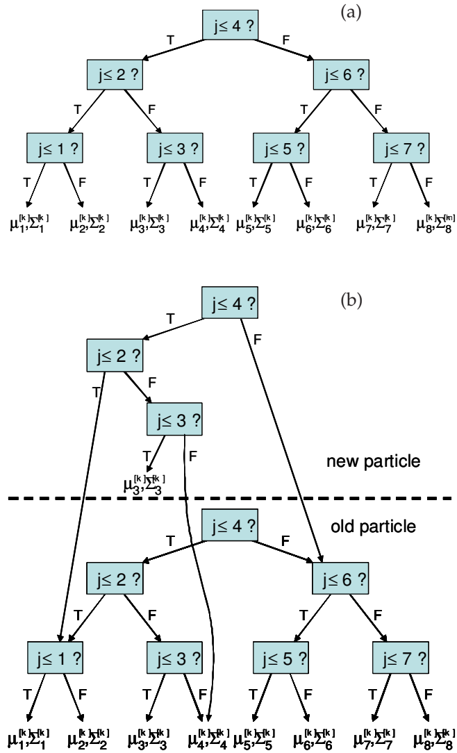
Figure 13.8 (a) A tree representing N = 8 feature estimates within a single particle. (b) Generating a new particle from an old one, while modifying only a single Gaussian. The new particle receives only a partial tree, consisting of a path to the modified Gaussian. All other pointers are copied from the generating tree. This can be done in time logarithmic in N .
